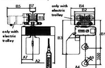
Chain hoist with trolley
